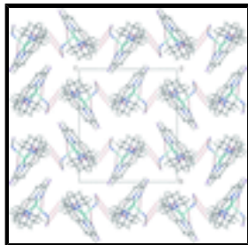
Fig. 2. The packing diagram of the title compound, viewed down the crystallographic a axis.
